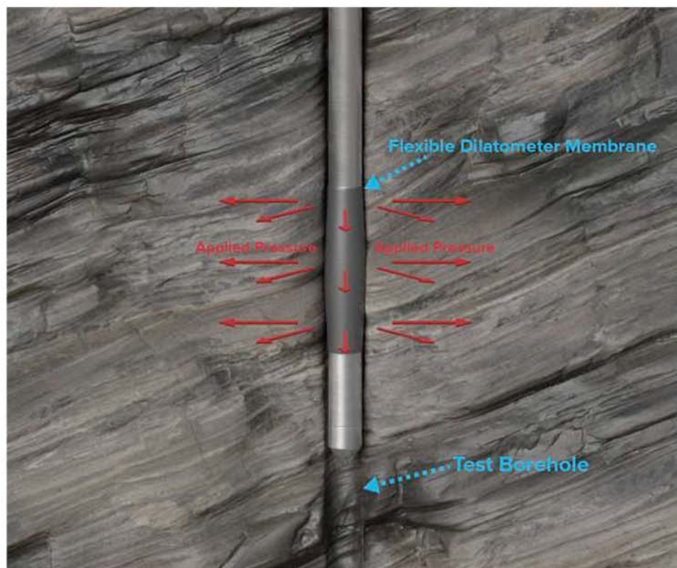
FIG. 1 General Depiction of a Flexible Dilatometer, Deflated (a) and Inflated (b) in a Borehole
