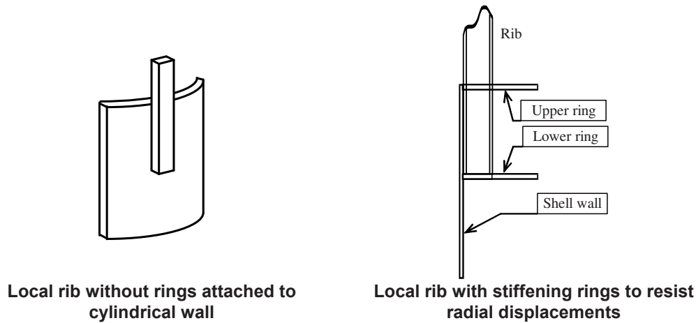
Figure 5.8: Typical details of loading rib attachments
