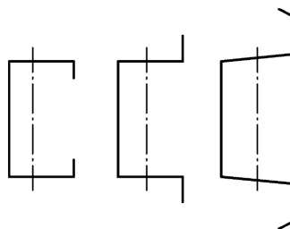
Figure 5.5 a): Cold-formed stiffeners with edge stiffened flanges EN 1993-1-3 identify s: buckling curve b
