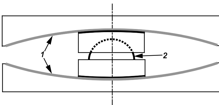
Figure 5 — Double Curved Surface Slider without hinge
