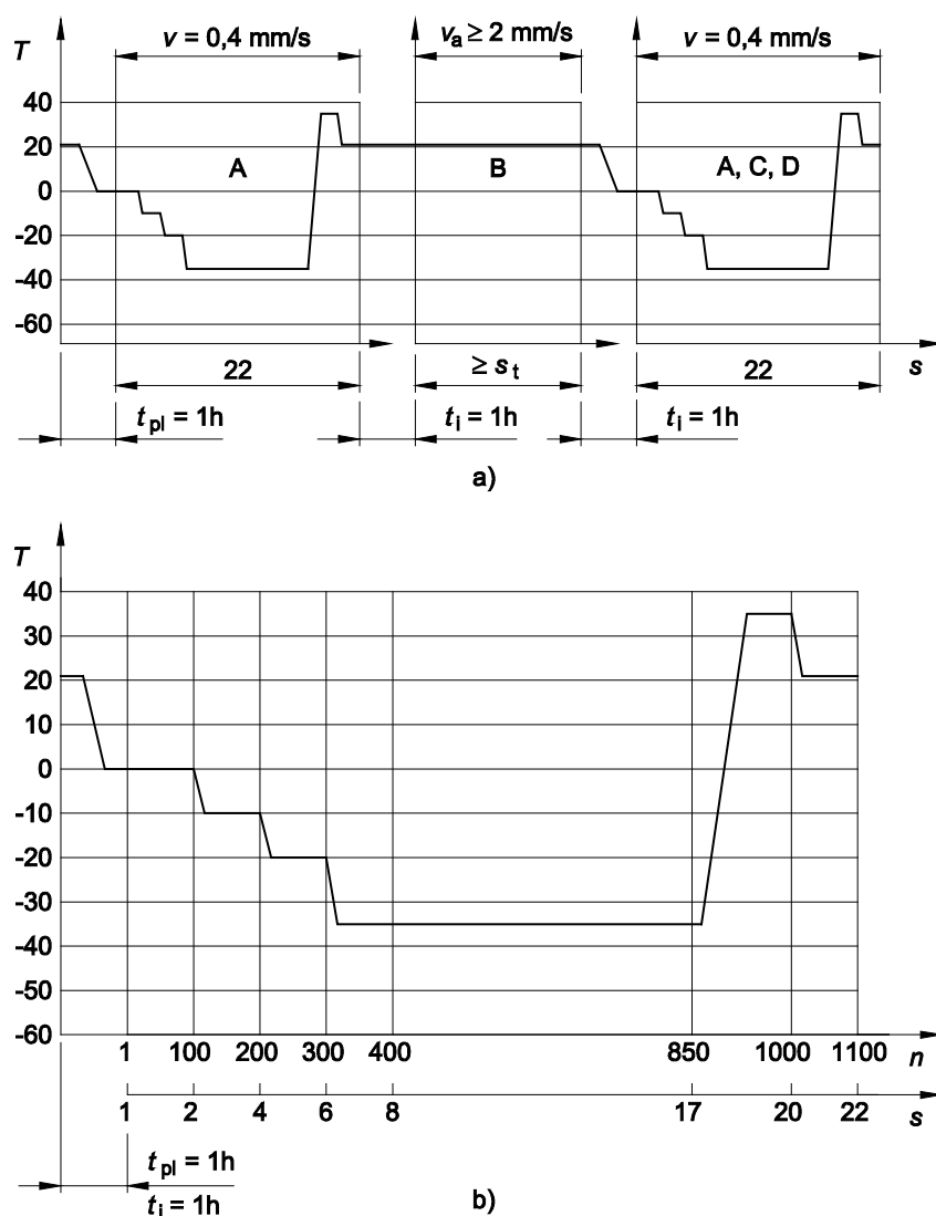
Figure 7 — Temperature profile of the long-term sliding test
